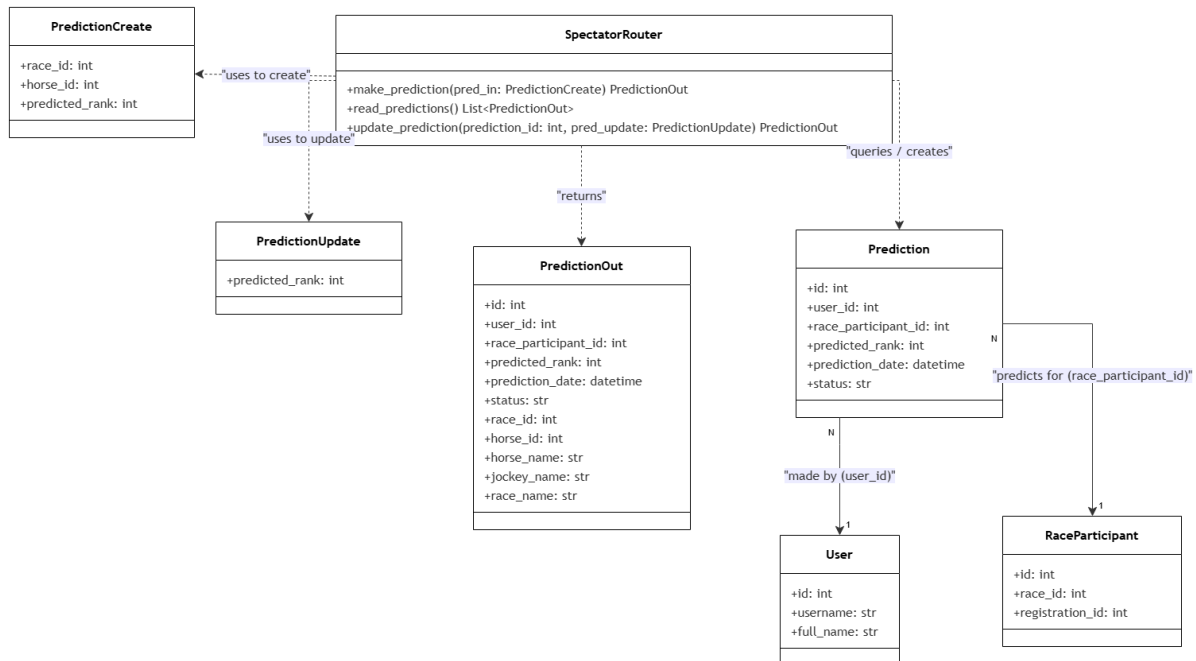
Figure 4.7: Spectator Prediction Class Diagram
