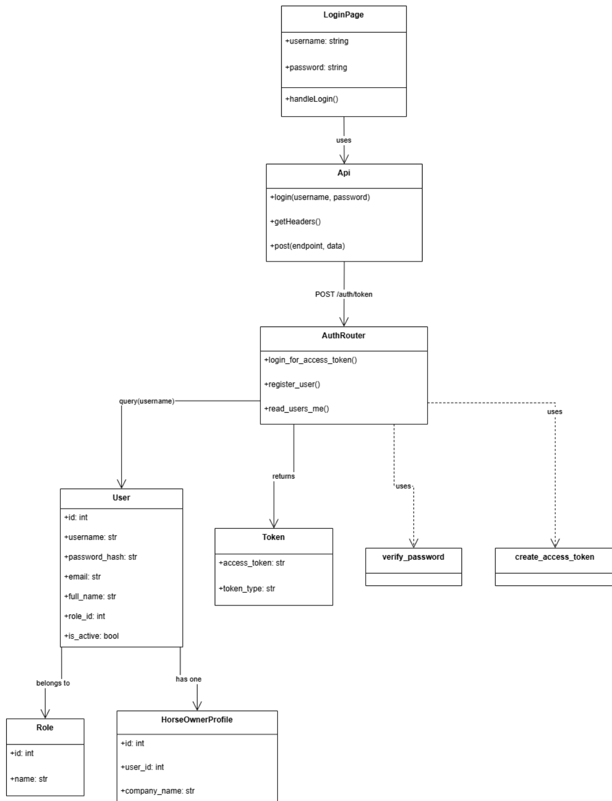
Figure 4.1: Login Class Diagram
