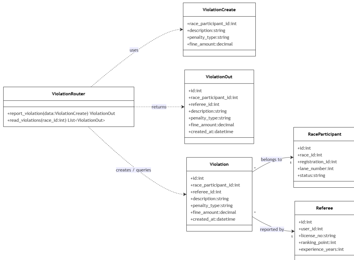
Figure 4.59: Violation Report Class Diagram
