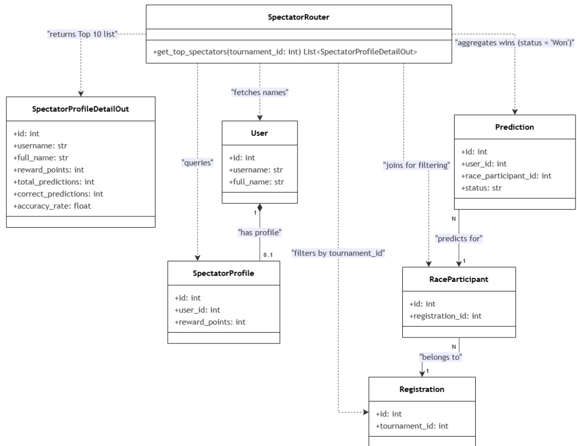
Figure 4.51: Top 10 Spectators Leaderboard Class Diagram
