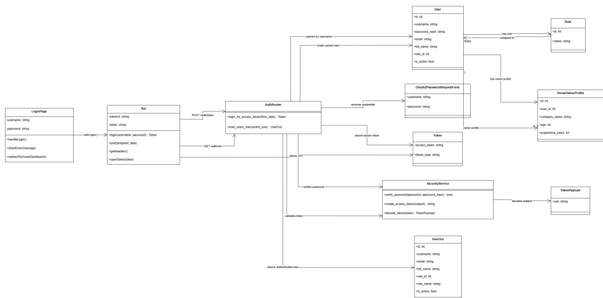
Figure 4.9: Horse Owner Authentication and Authorization Class Diagram
