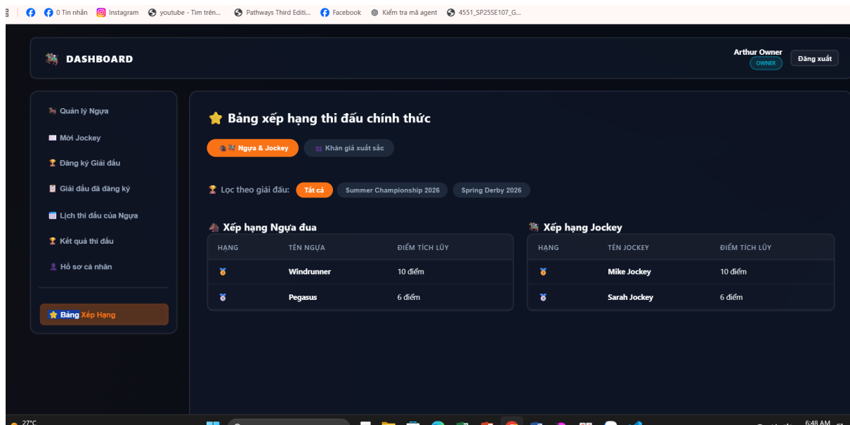
Figure 3.11: Ranking
