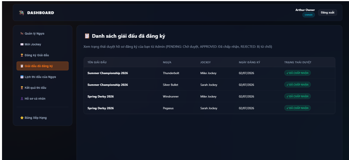
Figure 3.7: Registered Tournaments
