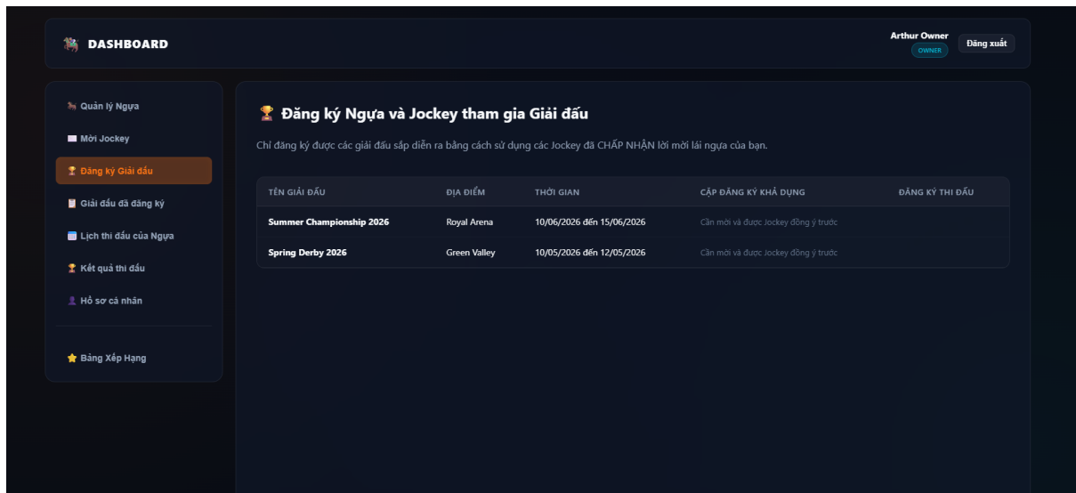
Figure 3.6: Tournament Registration
