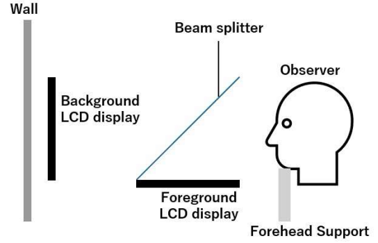
Fig. 3: Schematic diagram of experiment
