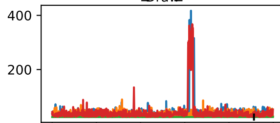
c_rpo_0 Draw
