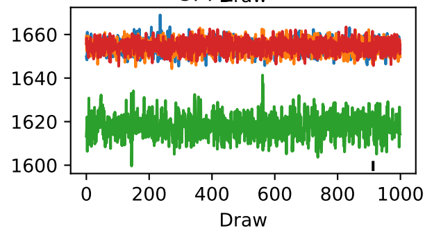
gpp_anual Draw
