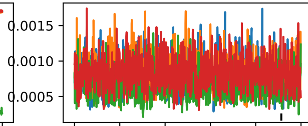
c_rpo_0 Draw
