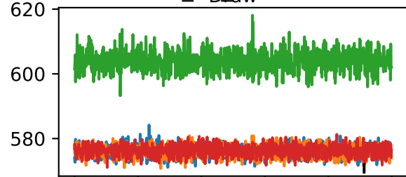
gpp_anual Draw
