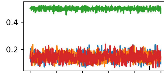
c_wco_0 Draw
