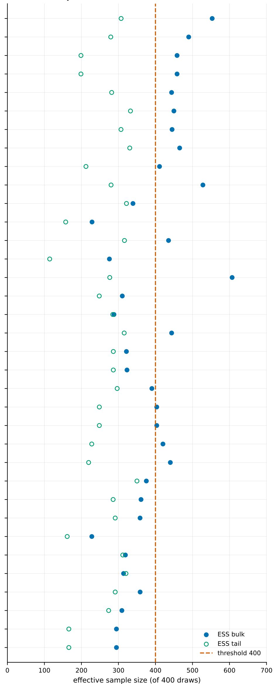
Effective sample size
