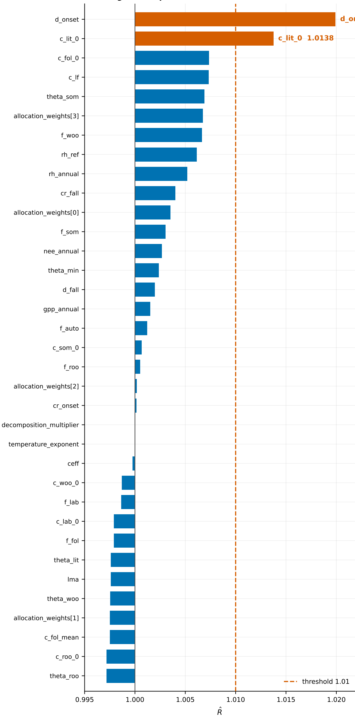
Convergence: \hat{R} per variable
