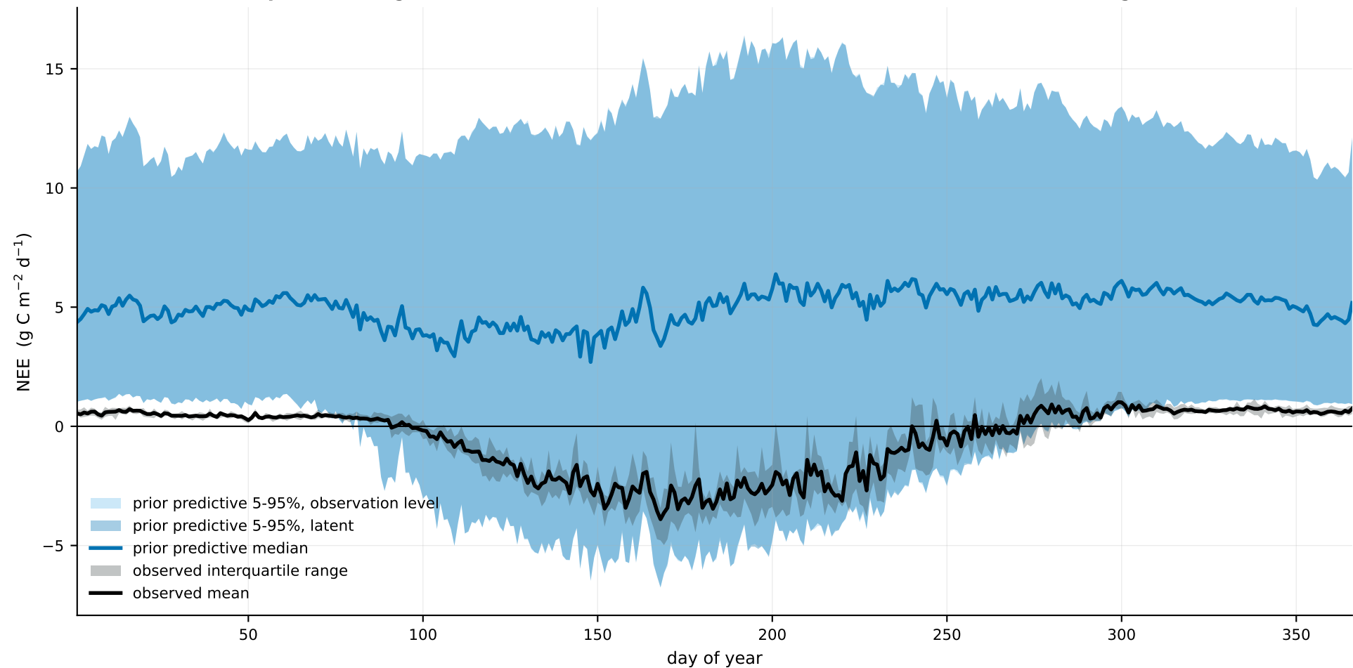
fig02 -- mean seasonal cycle, prior predictive check
