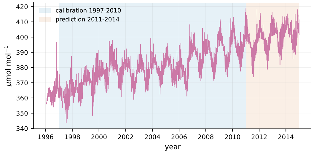
CO2_F_MDS, atmospheric CO 2
