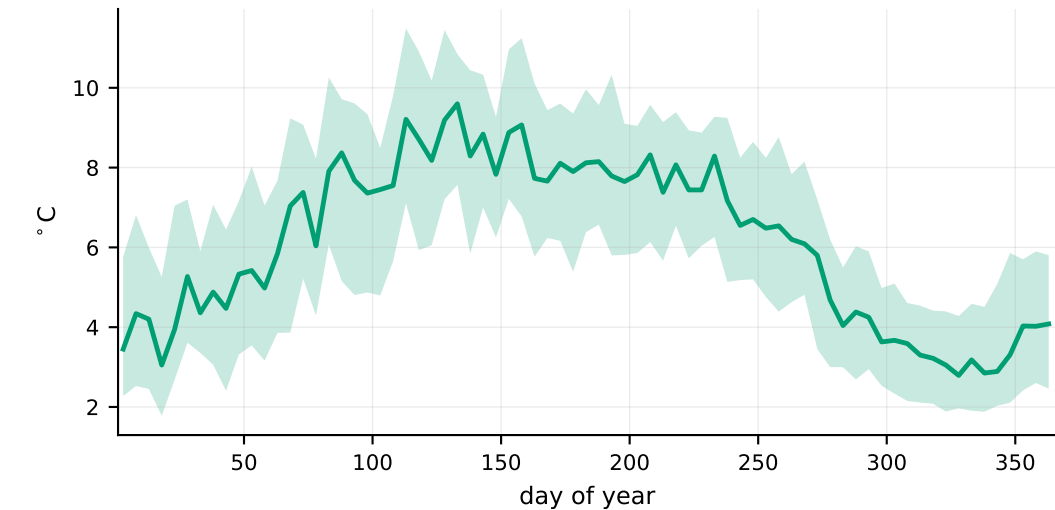
daily temperature range, from half-hourly
