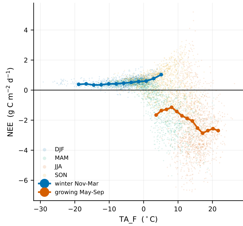
NEE vs temperature, binned by season
