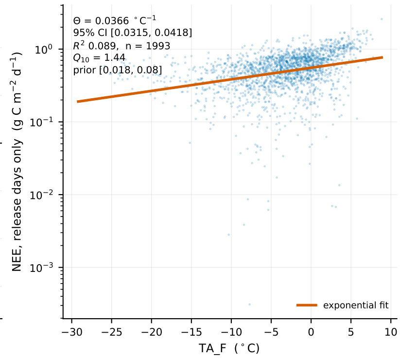
Winter respiration response
