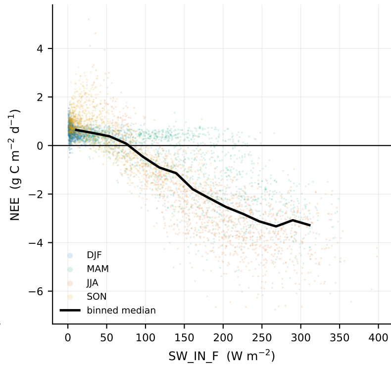
NEE vs incoming shortwave
