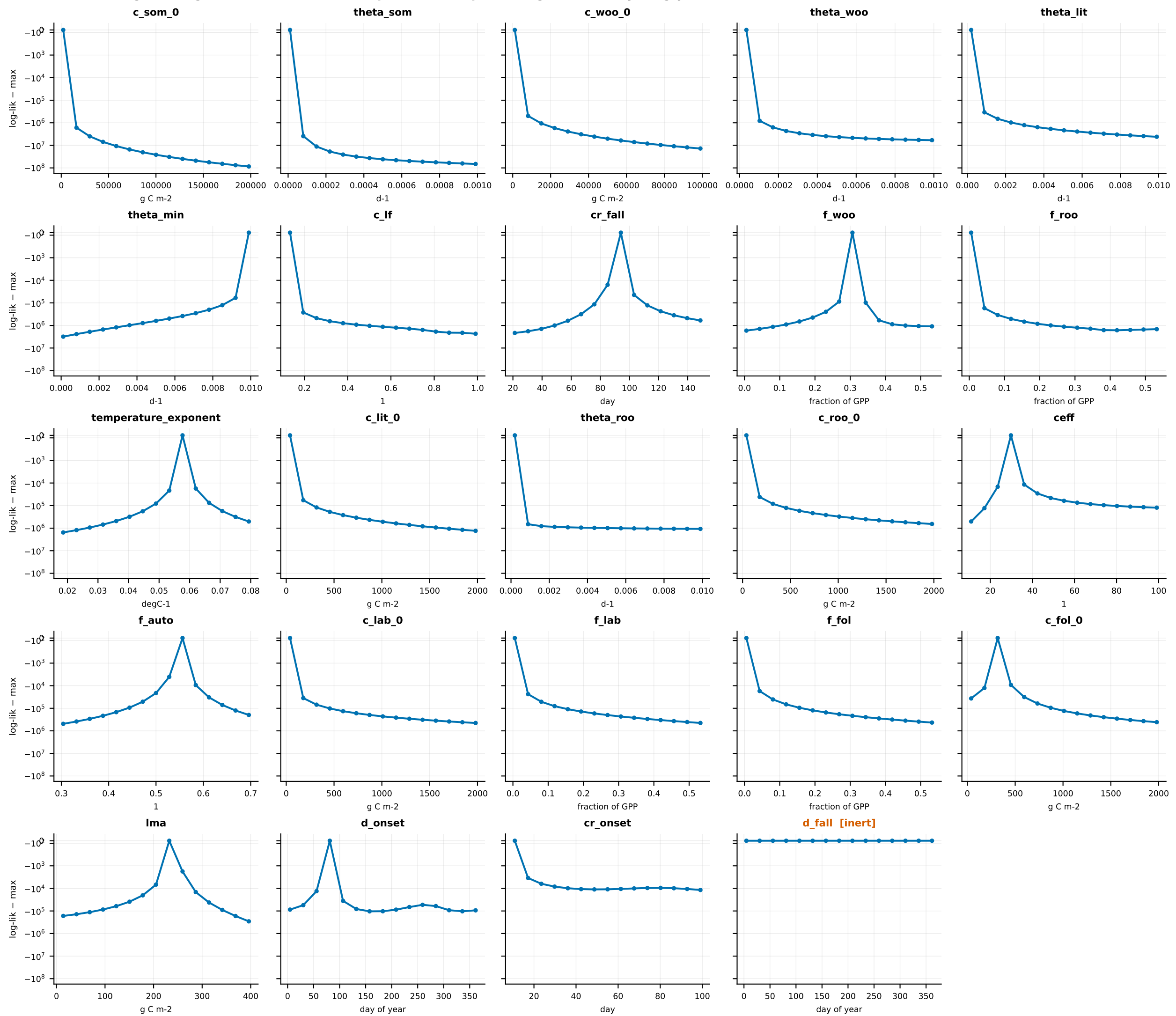
fig05 -- log-likelihood across each parameter's prior range, shared symlog y-axis (anchor: median of 163 usable Task 1 draws)
