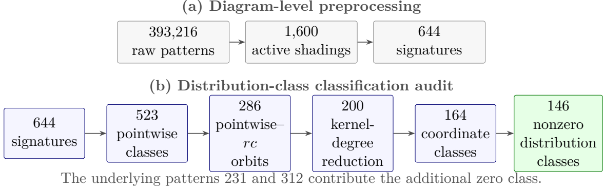
Figure 1: The two levels of the classification. Panel (a) records the diagram-level preprocessing. Panel (b) gives the distribution-classification audit; its arrows represent, from left to right, pointwise equality, reverse-complement, kernel-degree reduction, layer-coordinate relabelling, and the remaining distributional bridges.
