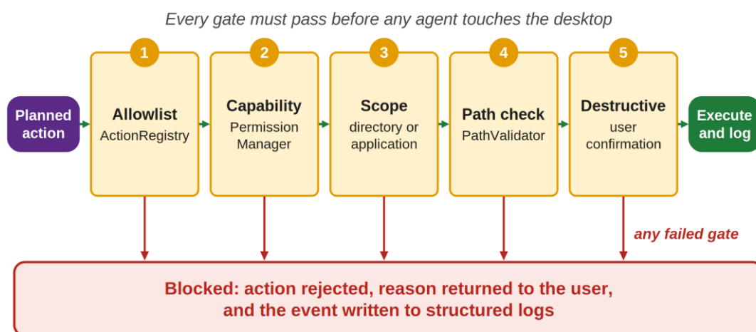
Figure 3.5 Security Validation Pipeline
