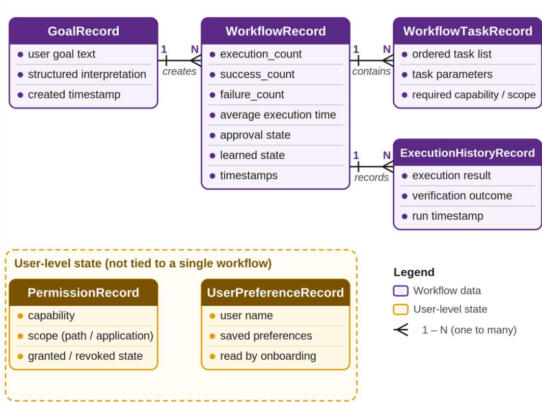
Figure 4.1 Persistent Data Model
