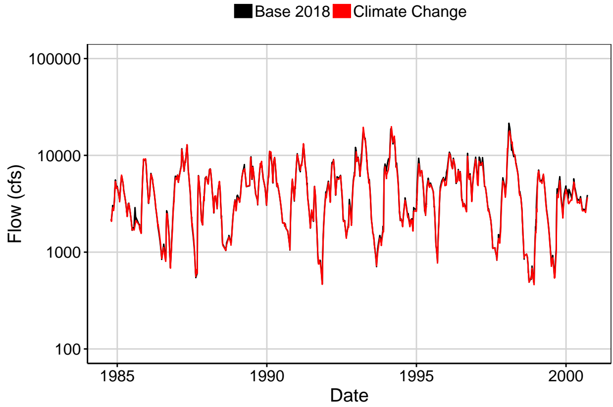
Fig. 4: Baseflow
