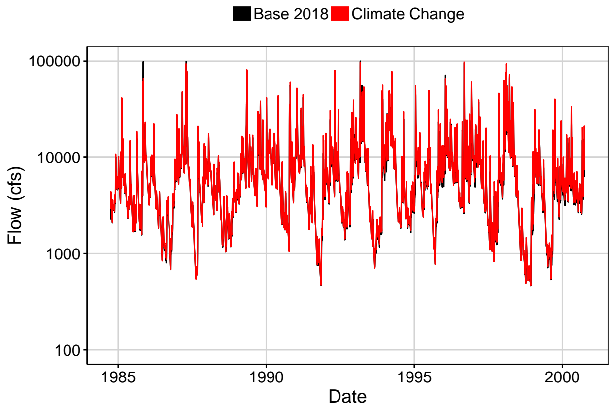
Fig. 1: Hydrograph
