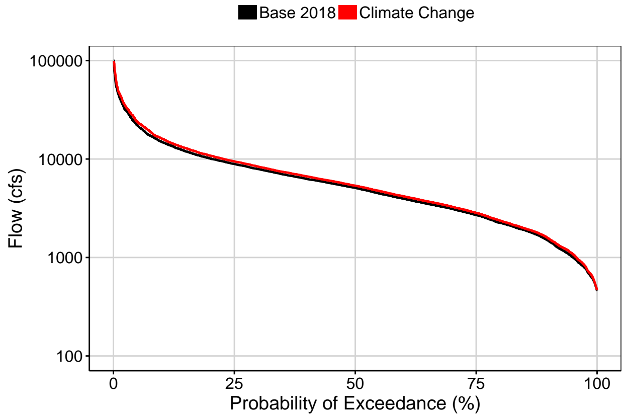
Fig. 3: Flow Exceedance
