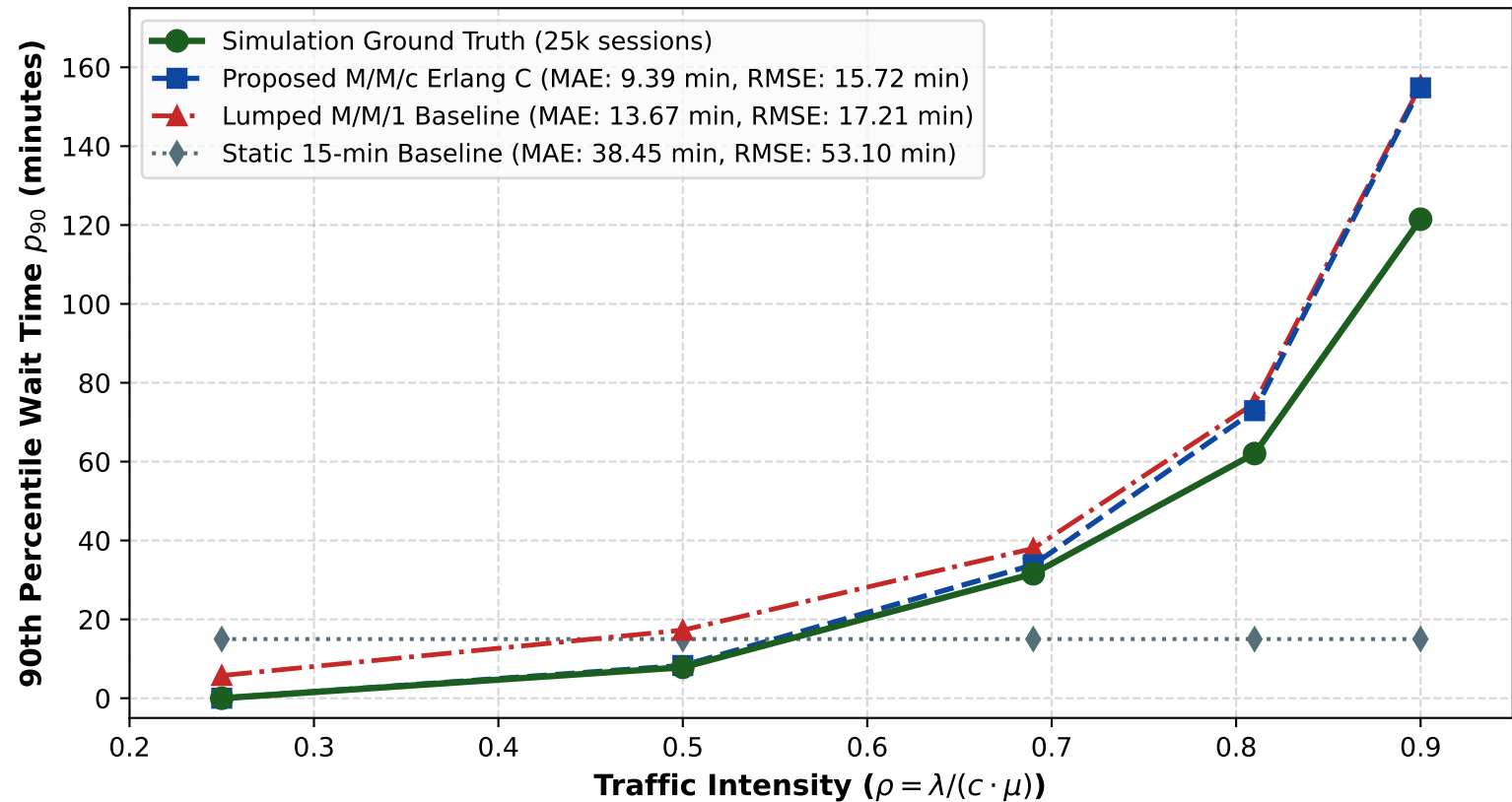
Comparative Tail Queue Delay ( p_{90} ) across Traffic Intensities ( c = 4 ports, \mu = 2.0 )
