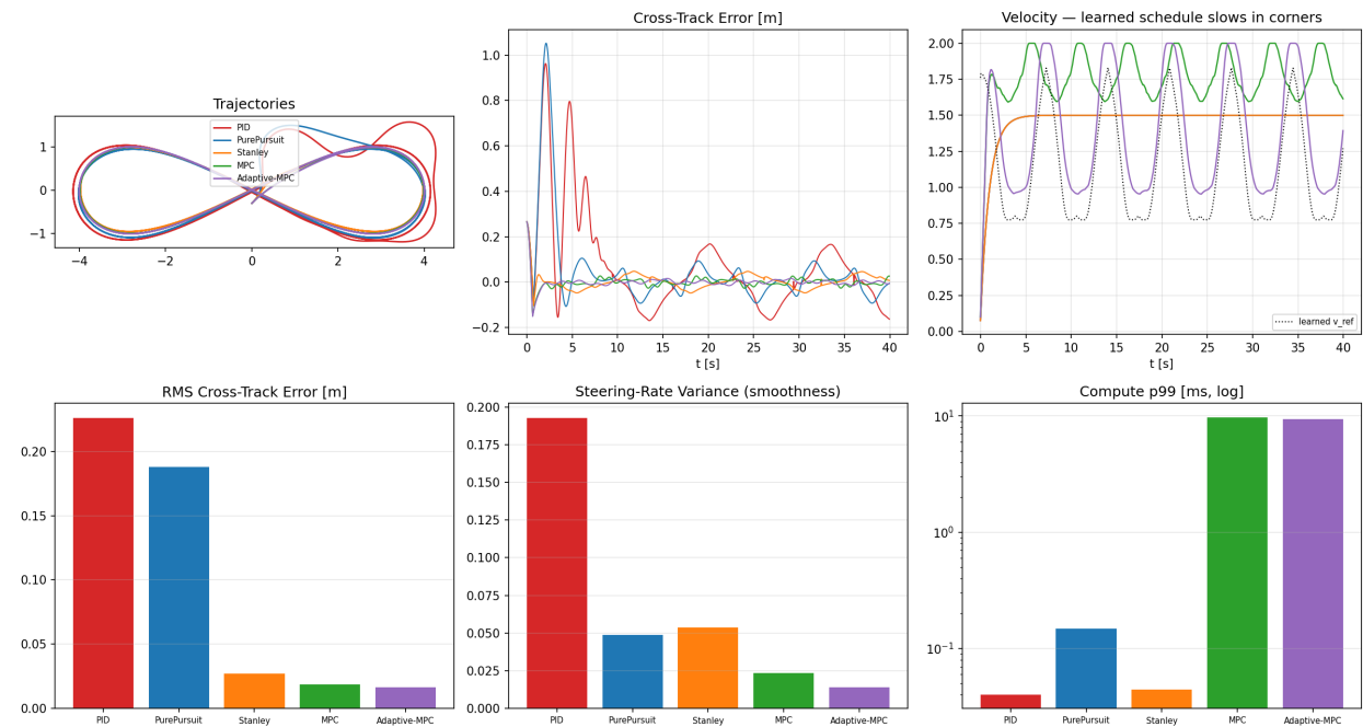
Figure 3: trajectories, cross-track error, velocity (with learned schedule), and metric bars.
