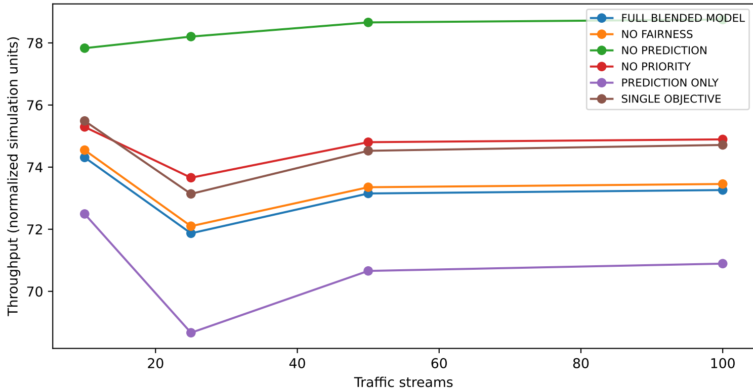
Ablation comparison
