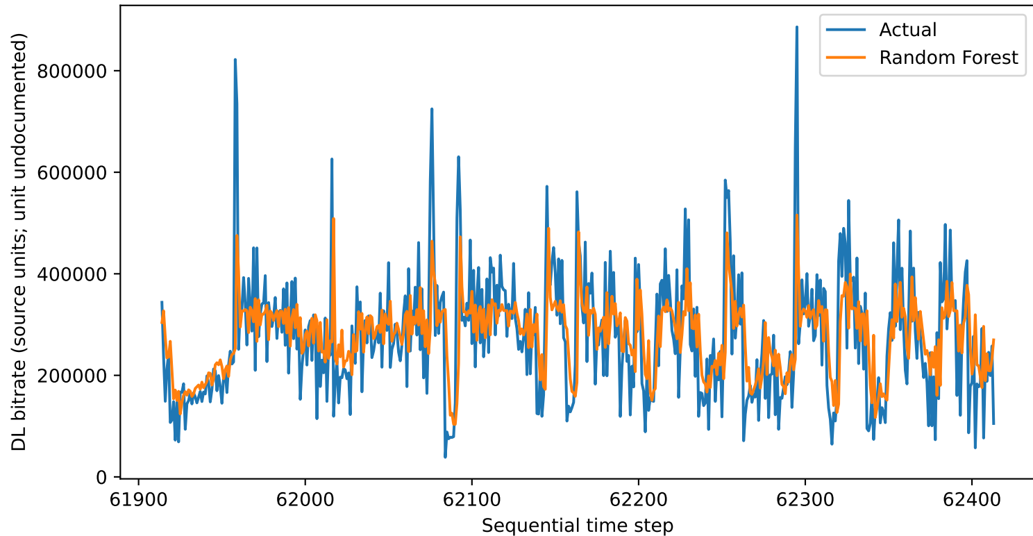
Actual and predicted DL demand: afreeca_dataset
