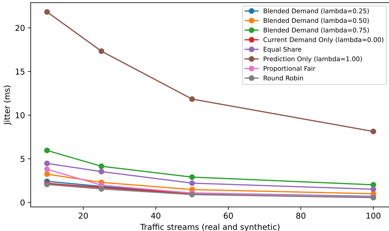
Jitter (ms) vs traffic stream count (high load)
