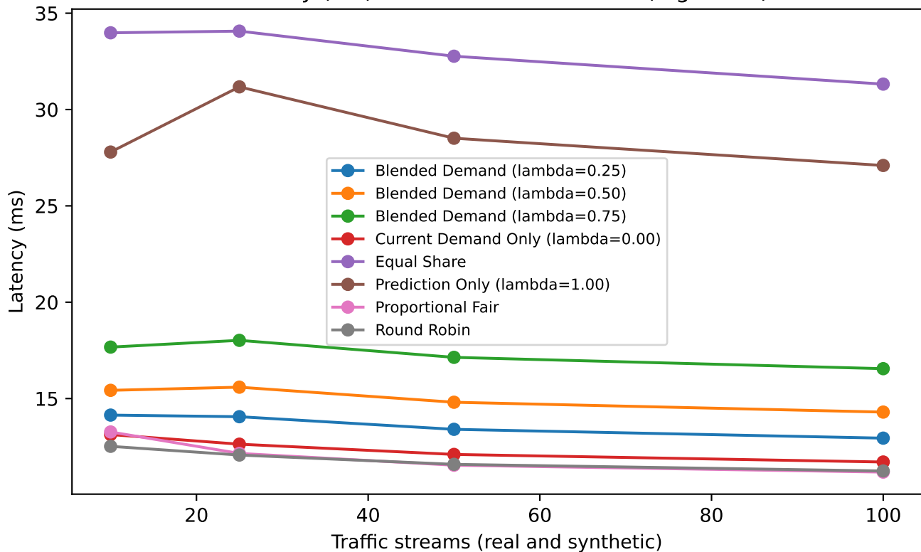
Latency (ms) vs traffic stream count (high load)
