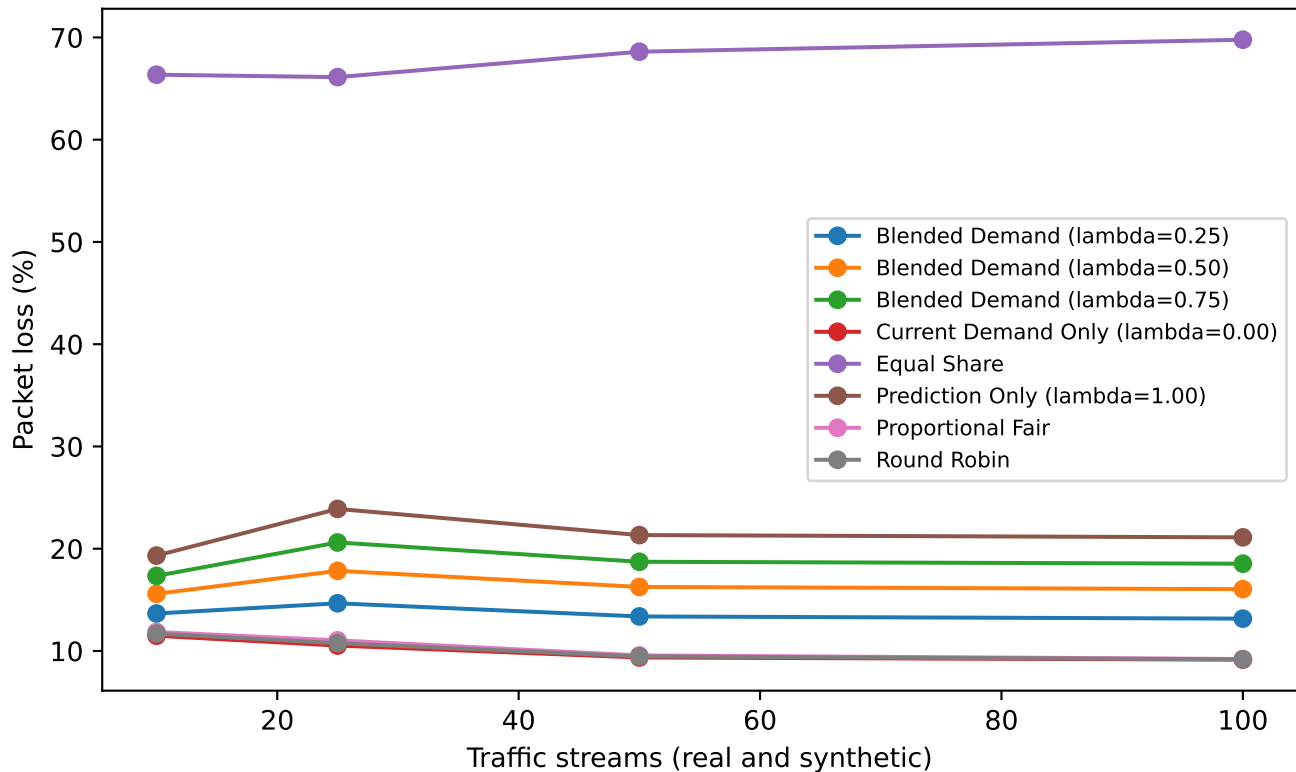
Packet loss (%) vs traffic stream count (high load)
