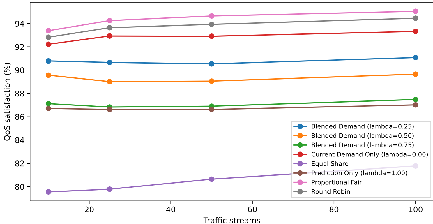
Blended (lambda=0.75) and baseline QoS comparison
