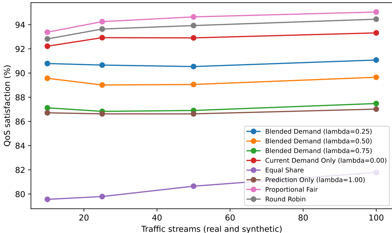
QoS satisfaction (%) vs traffic stream count (high load)
