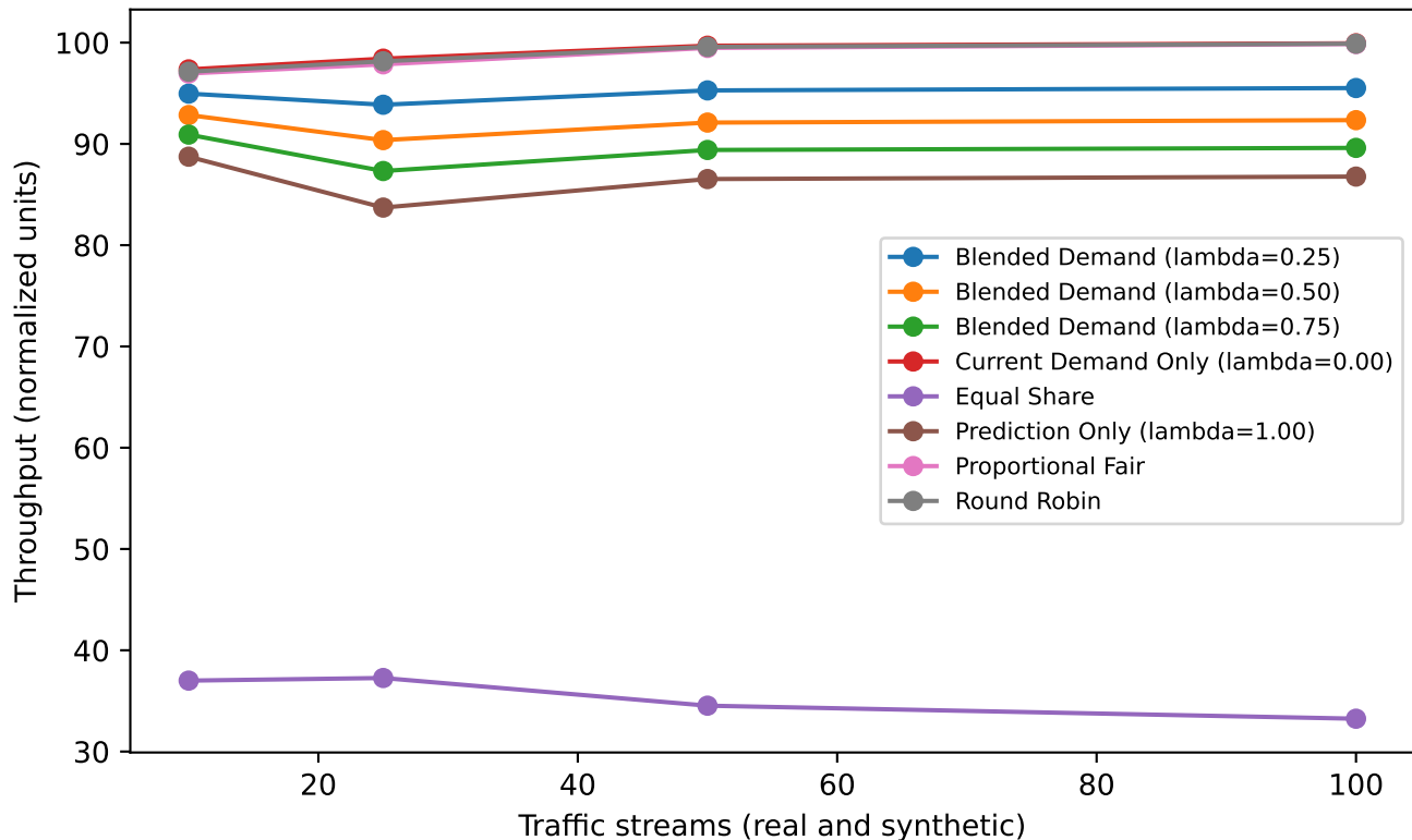
Throughput (normalized units) vs traffic stream count (high load)
