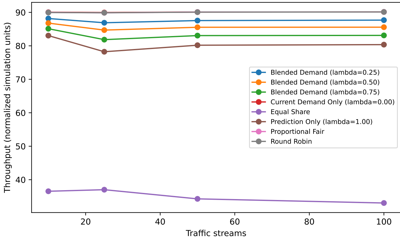
Throughput under traffic spike
