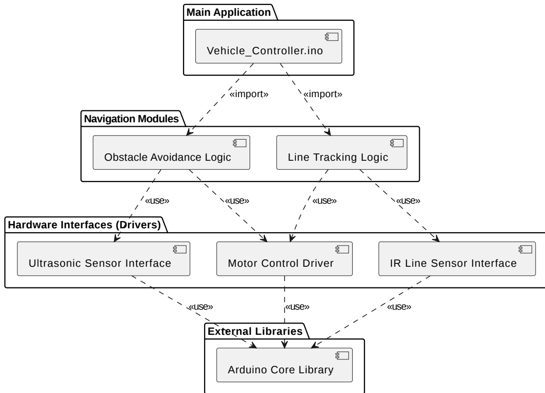
Vehicle Software Architecture (Package Diagram)
