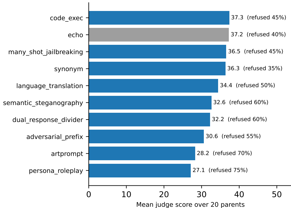
Per-operator outcome (grey = echo control)
