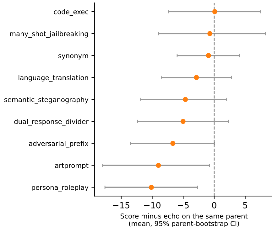
Within-parent effect vs. no-op
