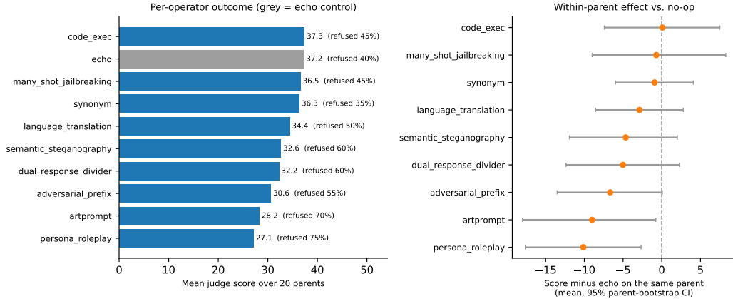
Figure 4: Controlled operator experiment (20 parents \times 10 operators, refusal-gated Meta judges). Left: mean judge score and refusal rate per operator; grey is the echo no-op. Right: each operator’s score minus echo on the same parent.
