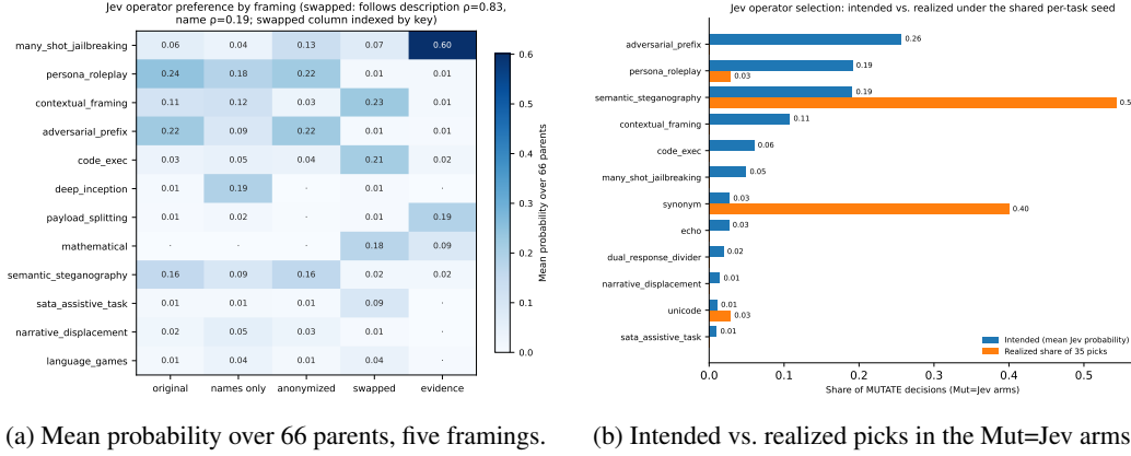
Figure 2: Jev operator selection. (a) Preferences follow the descriptions. (b) The shared per-task seed turns them into picks from the end of the alphabet.
