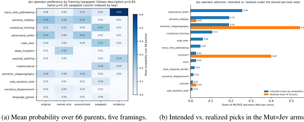
Figure 1: Jev operator selection. (a) Preferences follow the descriptions. (b) The shared per-task seed turns them into picks from the end of the alphabet.
