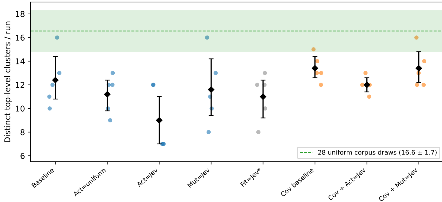
Corpus-cluster breadth per run (dots = seeds, \blacklozenge = mean, 95% seed-bootstrap CI)
