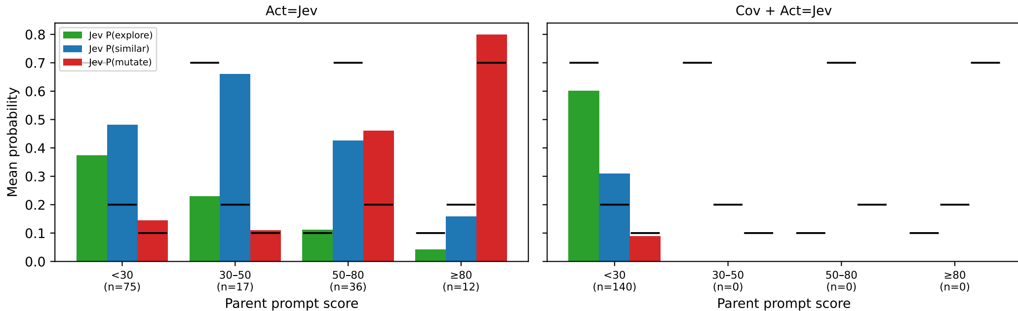
Jev action probabilities vs. parent score (bars) against the static-threshold policy (black ticks)
