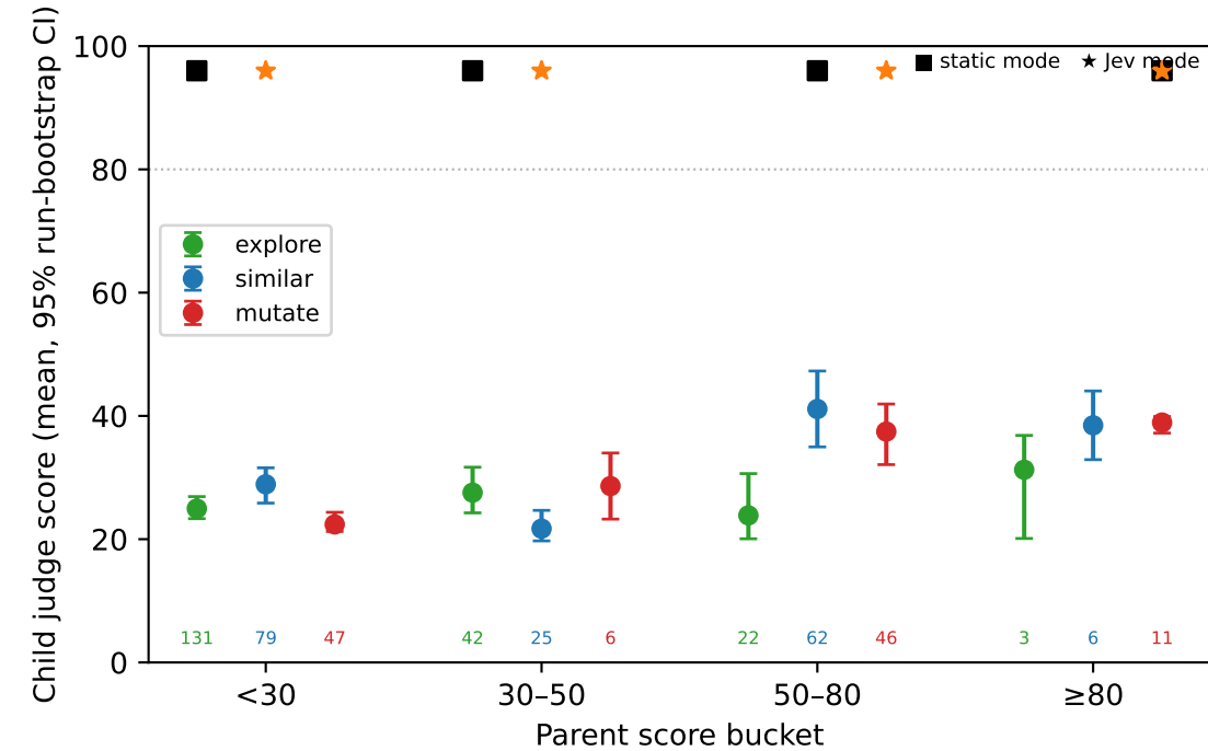
What each action produces, by parent score (pooled over Baseline, Act=uniform, Act=Jev, Mut=Jev; iterations \geq 1 ; n above x-axis)
