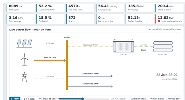
Figure 4.1 – Without battery at 22:00: 19.2 MW of wind less 4.0 MW of auxiliaries is below the 19.0 MW minimum load of the 19 modules in service; the electrolyser stops and 15.2 MW of wind power is curtailed.
