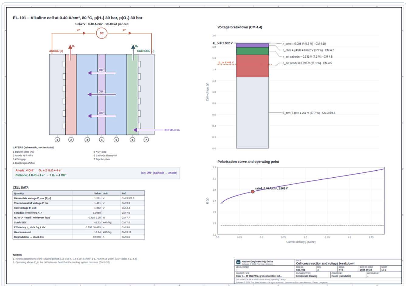
Figure 2.3 – CEL-001 for the alkaline cell of Case A.
