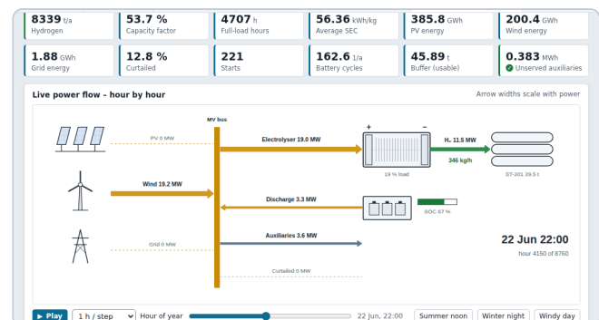
Figure 4.2 – With 30 MW / 60 MWh: the battery discharges 3.3 MW and keeps the electrolyser at its minimum load of 19.0 MW.
