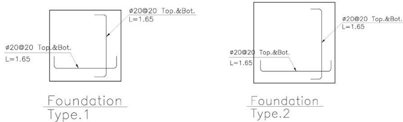
Foundation Plan
