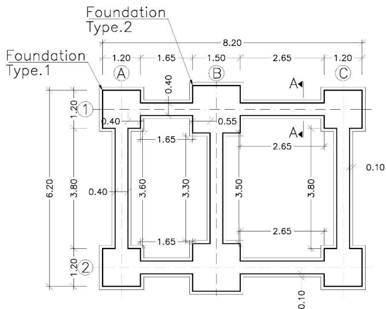
Foundation Plan
