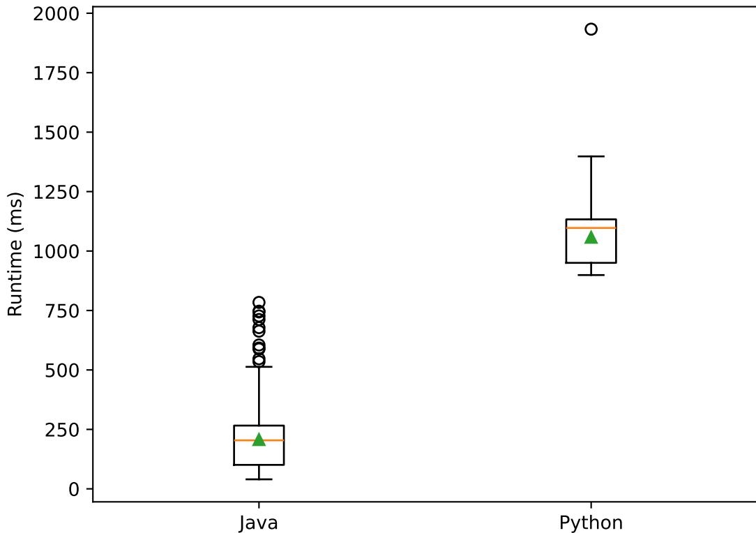
Runtime distribution (all included dataset sizes)
