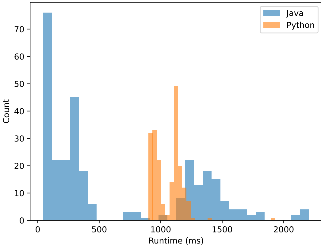
Runtime histogram
