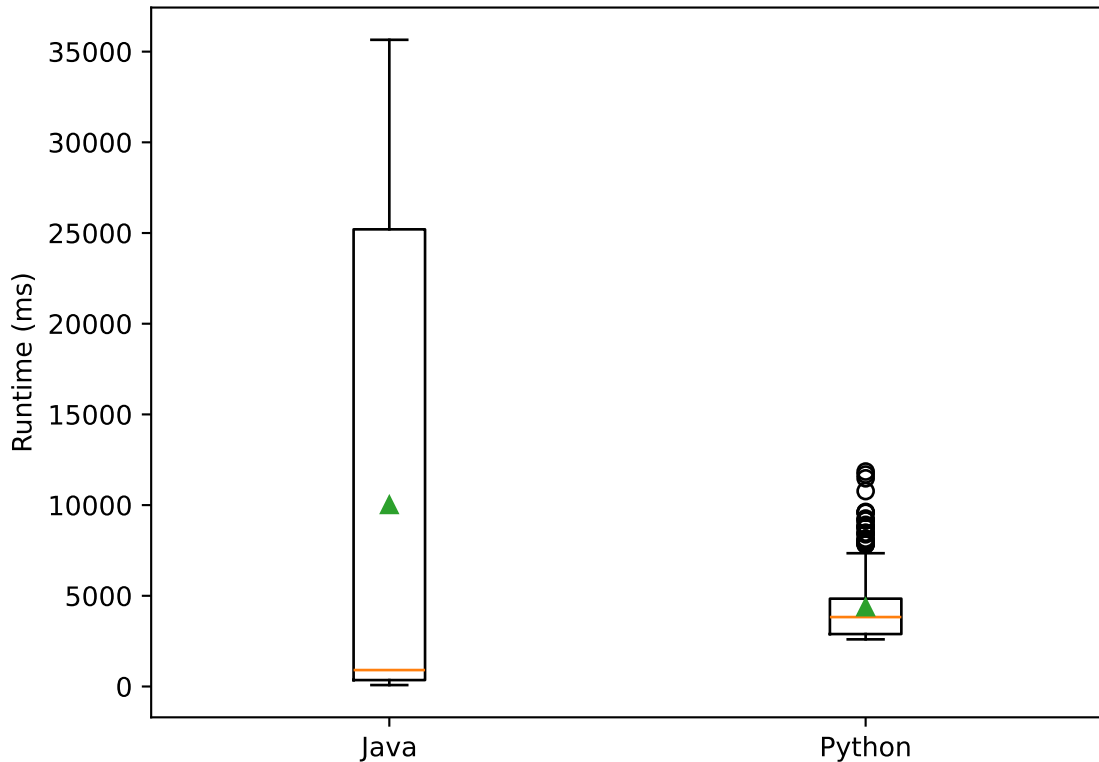
Runtime distribution (all included dataset sizes)
