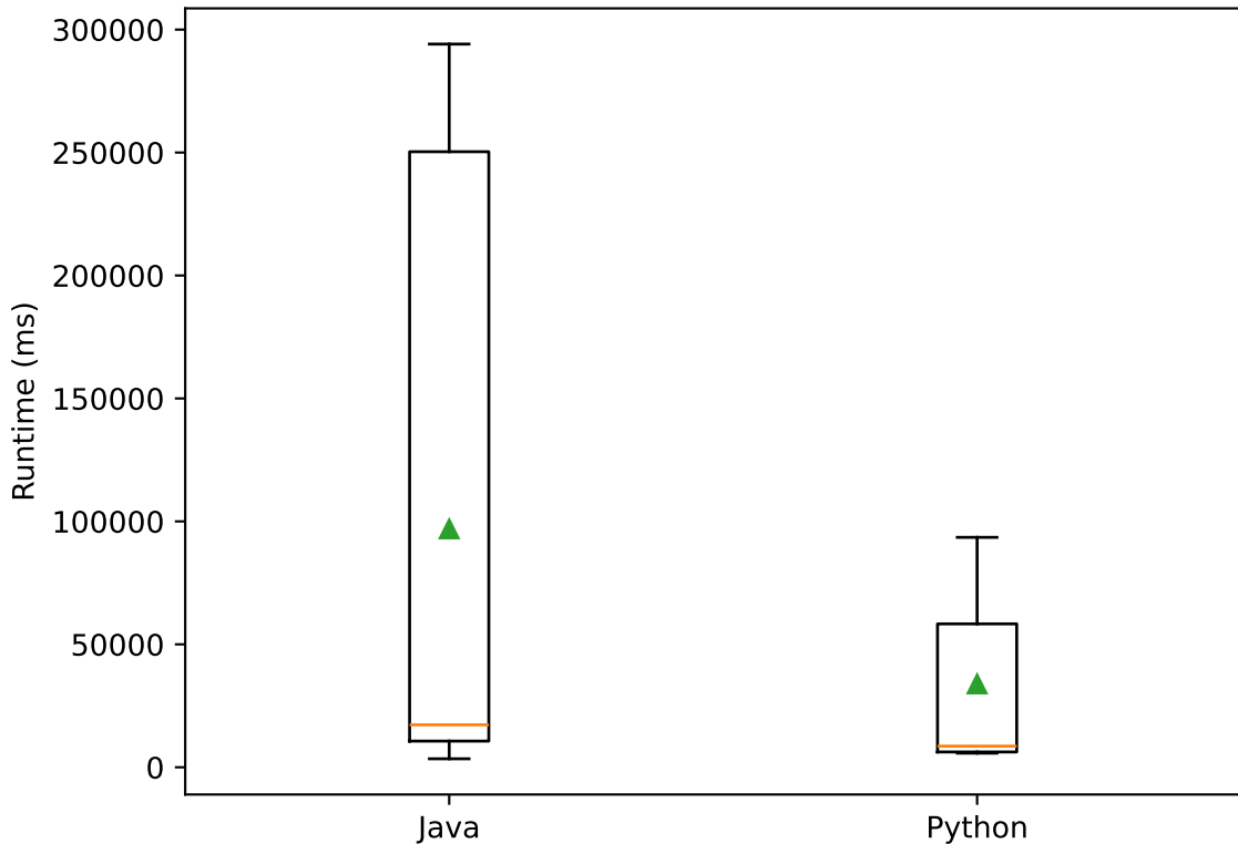
Runtime distribution (all included dataset sizes)
