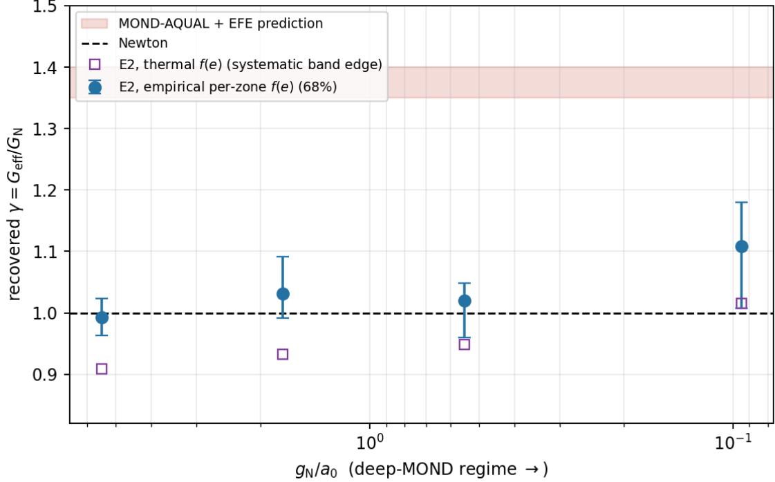
Figure 3: Recovered \gamma versus internal Newtonian acceleration (E2, perspective-corrected, fiducial cuts). Circles: empirical per-zone f(e) with 68% bootstrap intervals; open squares: thermal f(e) (lower edge of the systematic band). The MOND-AQUAL + EFE prediction (shaded) is excluded across the full acceleration range.
