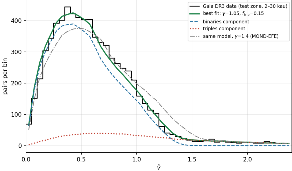
Figure 2: Test-zone (2–30 kau) \tilde{v} histogram of the fiducial Gaia DR3 sample versus the joint (\gamma, f_{\text{trip}}) mixture fit and its components. The grey dash-dotted curve keeps the best-fit f_{\text{trip}} and triple component fixed and rescales only the binary component to \gamma = 1.4 (triple inner velocities are high-acceleration and carry no EFE boost); it is rejected at \Delta \ln \mathcal{L} = 129 .
