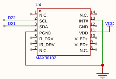
MAX30102
