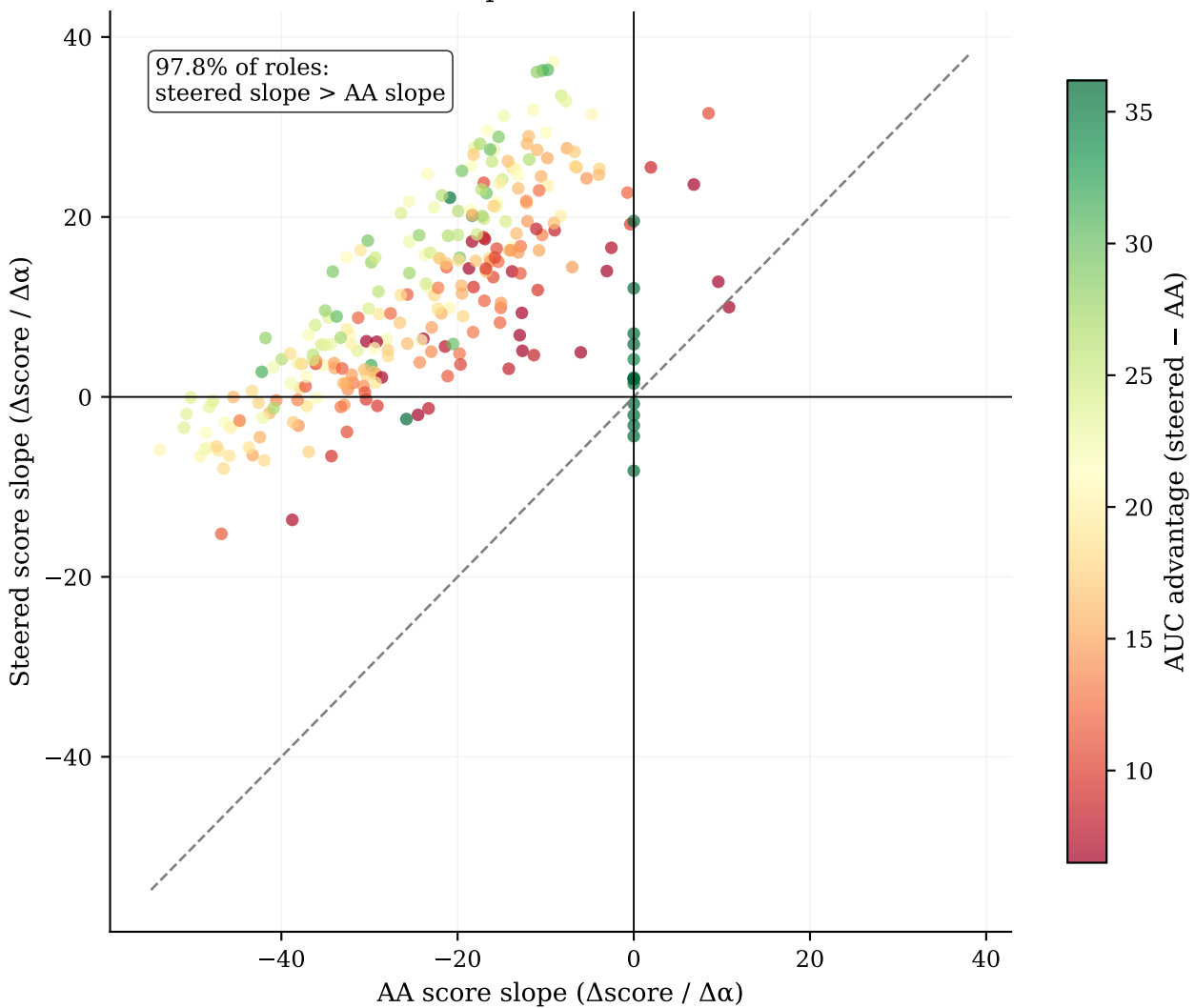
Per-role score slope: steered vs assistant axis
