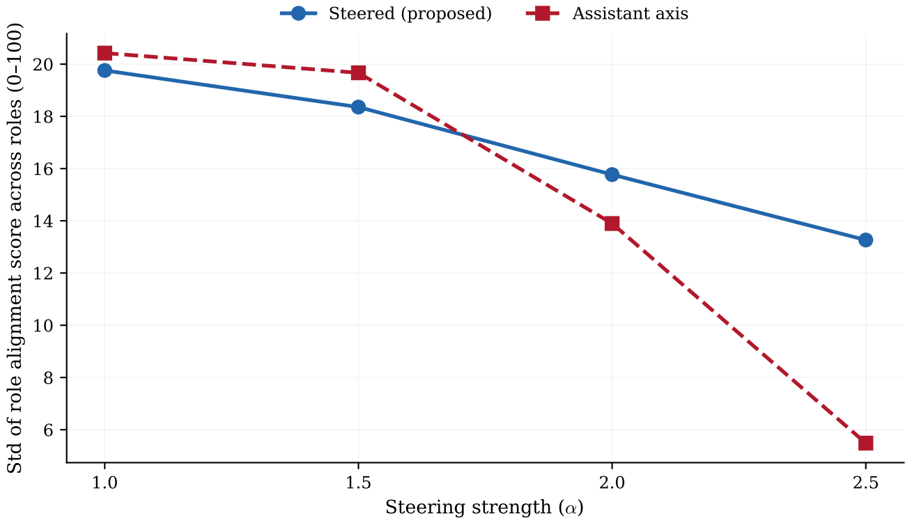
Inter-role score variance across 275 roles
