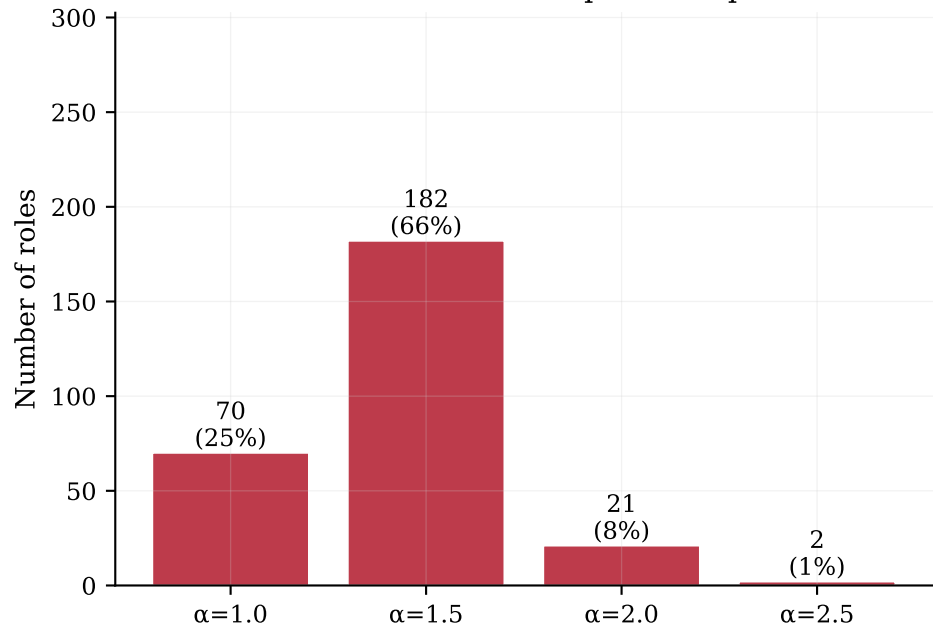
Assistant Axis: which alpha is its peak?
