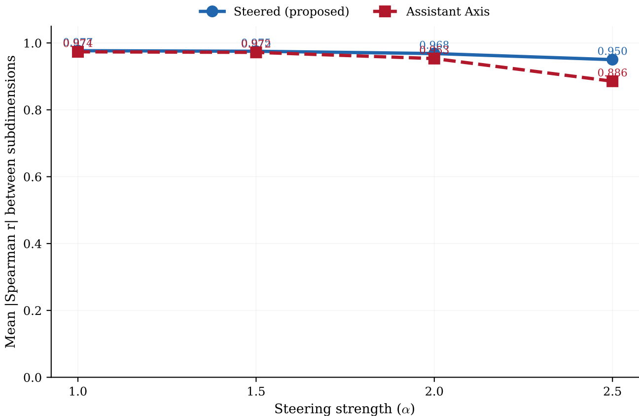
Subdimension inter-correlation vs steering strength
