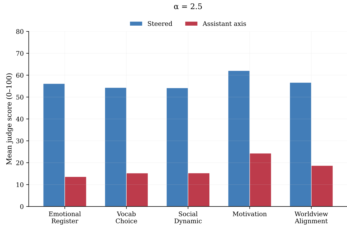
Mean sub-dimension scores: steered vs assistant axis
