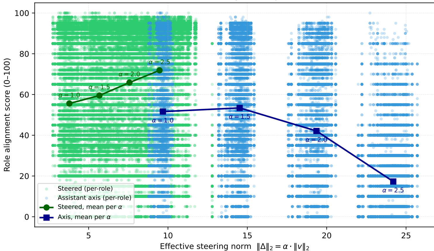
Score vs. Effective Steering Norm (per-role + means)
