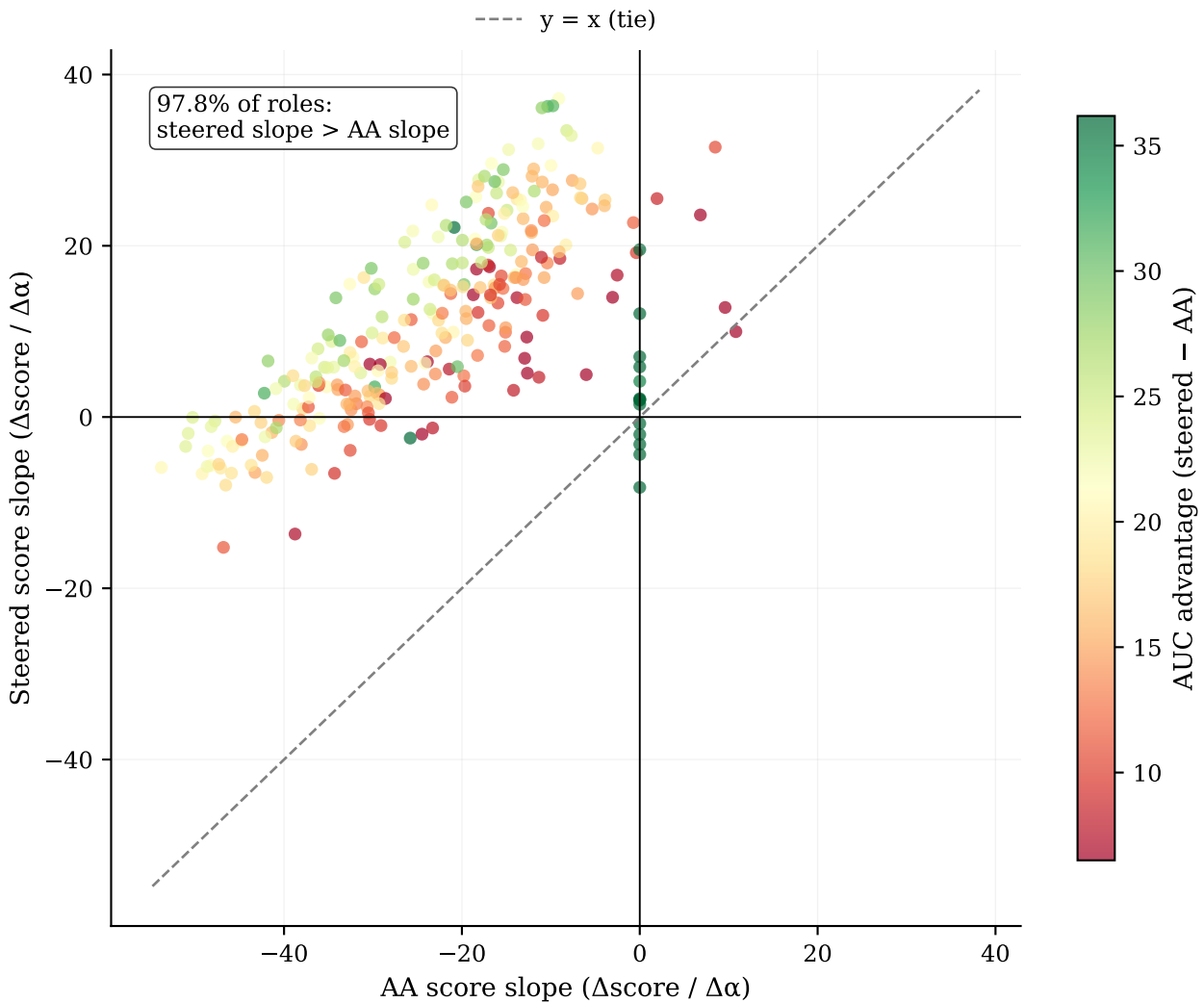
Per-role score slope: steered vs assistant axis
