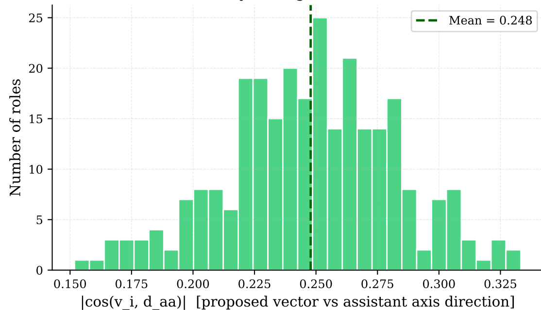
Alignment of proposed vectors with \mathbf{d}_{aa} (near 0 = nearly orthogonal to assistant axis)
