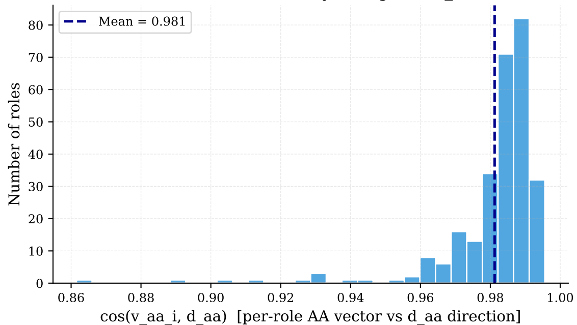
AA vector consistency with global \mathbf{d}_{aa}
